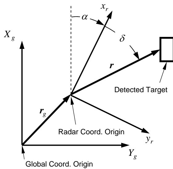
Figure A.1. Coordinate Systems for Radar Measurements.
