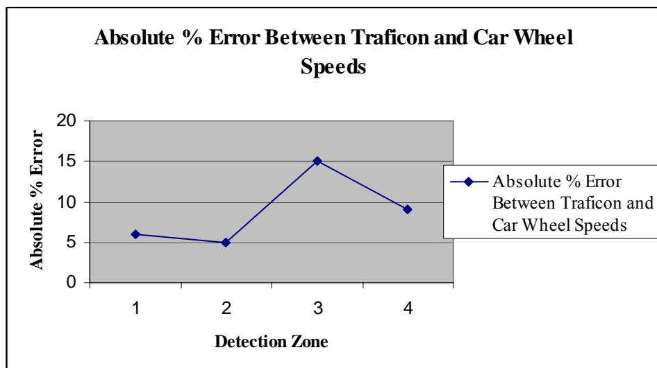
Figure 8.21 Absolute Percent Error between Traficon and Car Wheel Speed
